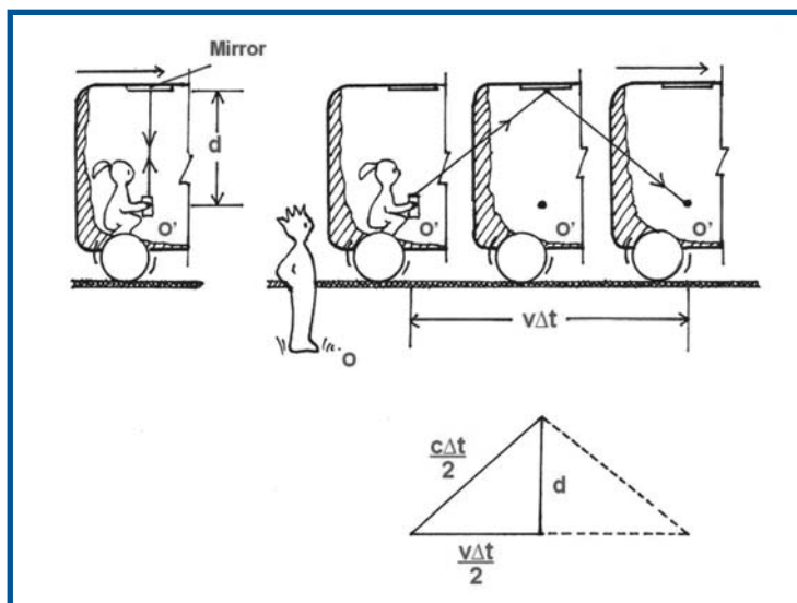
Fig. 6 A TE to show the time dilation effect - "moving clocks run slow".
