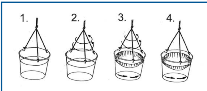
Fig. 3 Newton's "Rotating Bucket"
