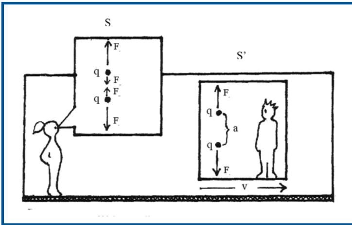
Fig. 9 Two electrons thought experiment.
