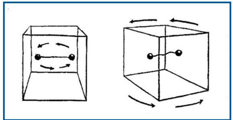
Fig. 4 Newton's two globes TE
